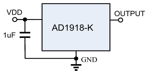
Figure 1, Typical Application Circuit of AD1918
