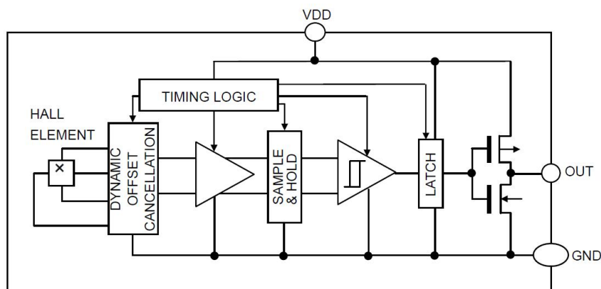
Figure 3, Block Diagram of AD1918
