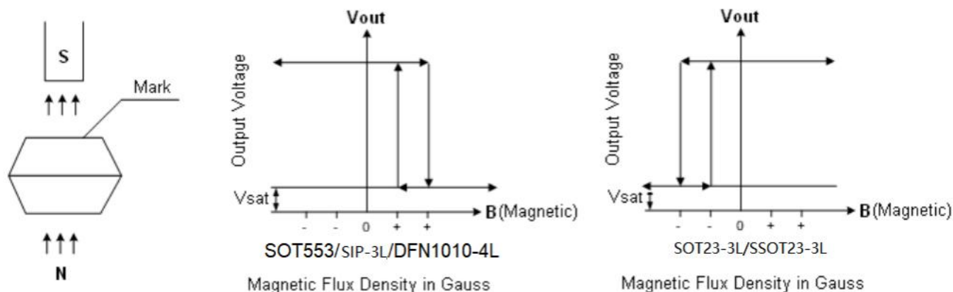
Fig 4, Magnetic Operation Characteristic of AD1918
